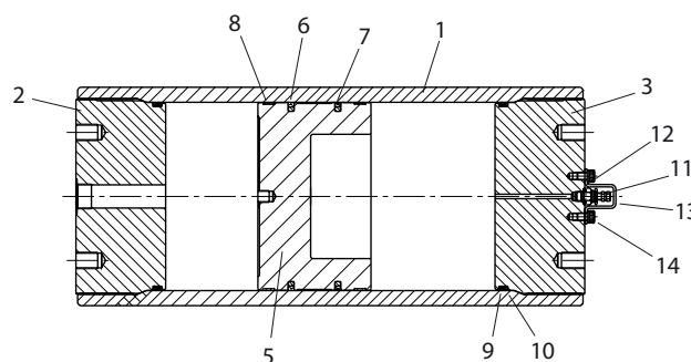
180mm and 250mm Bore Piston Accumulators
